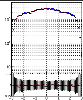
N of reco track vs \eta —•— Orig/DOM orig MS —+— pixelLess/DOM mod MS —x— pixelLess/DOM mod MS
