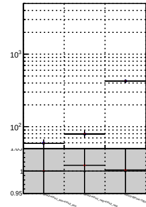
N of reco track vs. \chi^2 orig/DQM orig MS pixelLess/DQM mod MS pixelLess/DQM mod MS
