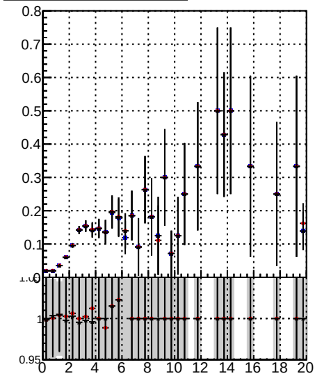
Fake rate vs. — Orig/DQM orig MS — pixelLess/DQM mod MS — pixelLess/DQM orig MS
