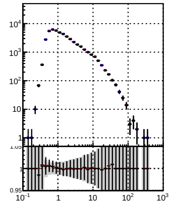
N of reco track vs \eta pixelLess/DQM mod MS pixelLess/DQM mod MS
