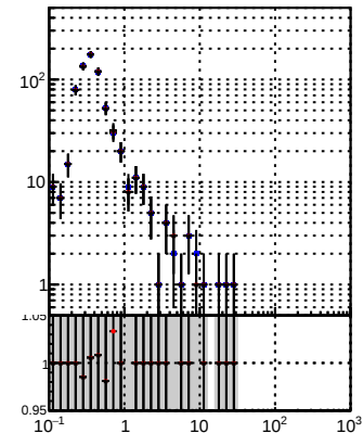
N of reco track vs \eta orig/DQM_orig_MS pixelLess/DQM_mod_MS orig/DQM_mod_MS
