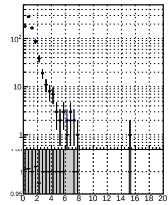
N of reco track vs. \chi^2 for pixel-less DOM mod MS
