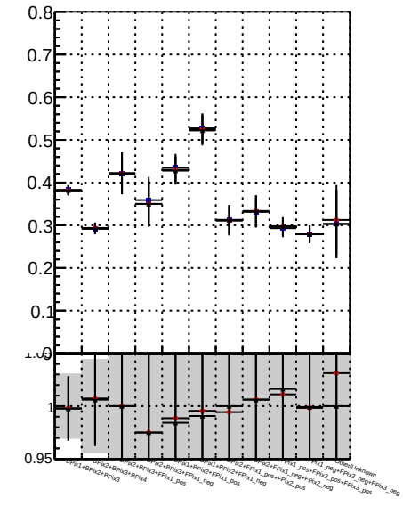
Fake rate vs. — pixelLess/DQM_mod MS — orig/DQM_mod MS — pixelLess/DQM MS
