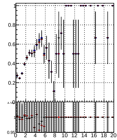
Fake rate vs. — pixelLess/DQM_mod MS — orig/DQM_mod MS — pixelLess/DQM MS
