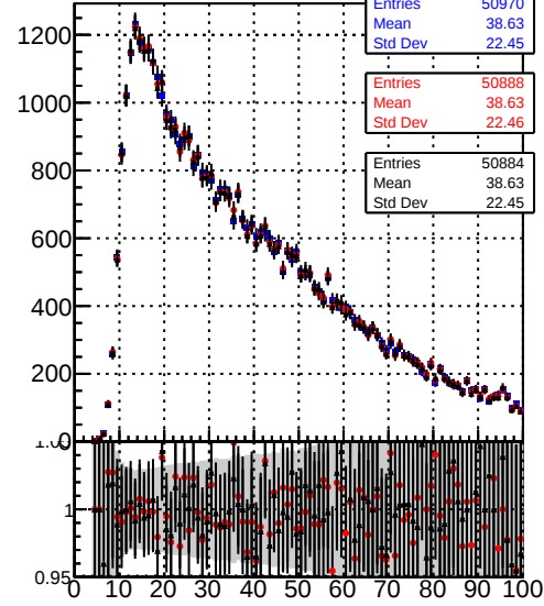
Uncertainty x Coordinate (other Vtx) - Legend: Orig/DQM_orig_MS (blue), pixelLessOrig/DQM_mod_MS (red), pixelLess/DQM_mod_MS (black)
