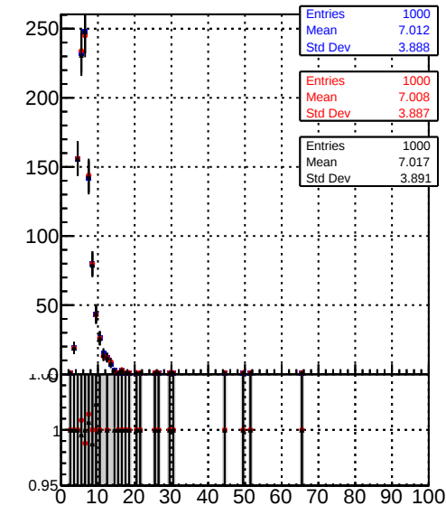
Uncertainty x Coordinate (other Vtx) - Legend: Orig/DQM_orig_MS (blue), pixelLessOrig/DQM_mod_MS (red), pixelLess/DQM_mod_MS (black)
