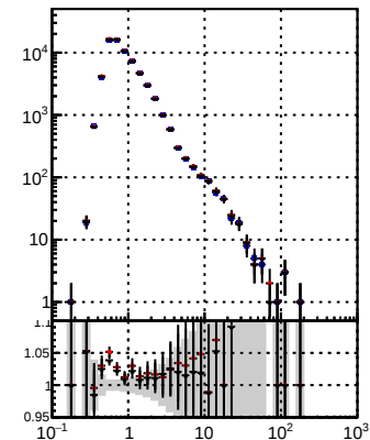
Orig/DQM_orig_MS pixelLess/DQM_mod_MS N of reco track vs pT
