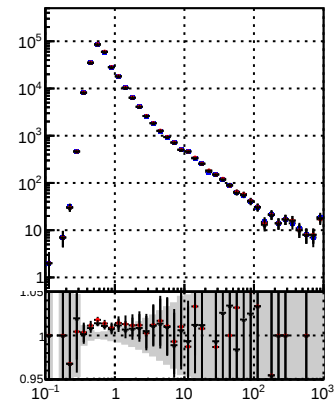
Orig/DQM_orig_MS pixelLess/DQM_mod_MS N of reco track vs pT
