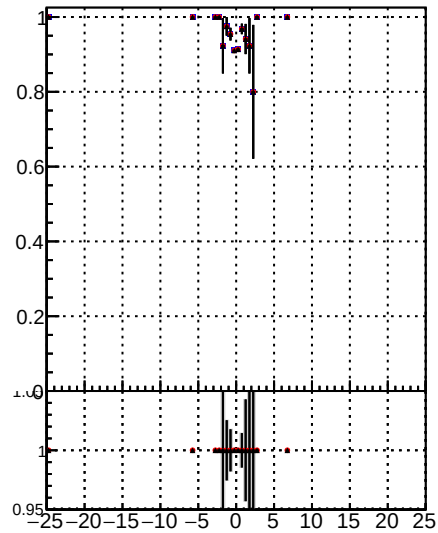
Fake rate vs d Orig/DQM_orig_MS pixelLess/DQM_mod_MS
