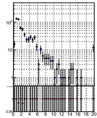
N of reco track vs. \chi^2 for pixel-less DQM model
