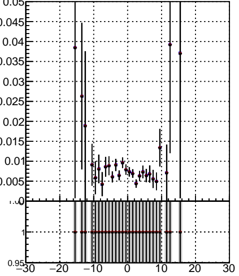
Efficiency vs sim PV z —•— Orig/DQM_orig_MS —•— pixelLessOrig/DQM_mod_MS —•— pixelLess/DQM_mod_MS
