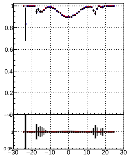
Fake rate vs d —•— Orig/DQM_orig_MS —•— pixelLess/DQM_mod_MS —•— pixelLess/DQM_mod_MS
