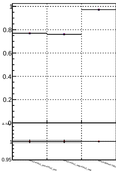
Fake rate vs. Orig/DQM_orig_MS pixelLess/DQM_mod_MS
