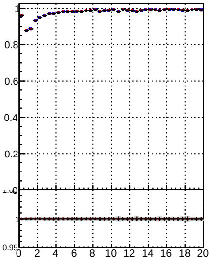
Fake rate vs. Orig/DQM_orig_MS pixelLess/DQM_mod_MS
