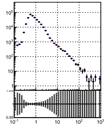
N of reco track vs pT N of associated (recoToSim) tracks vs pT N of associated (recoToSim) duplicate tracks vs pT
