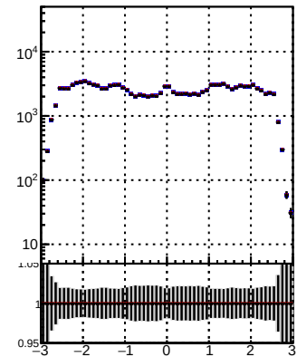
N of reco track vs \eta Orig/DQM orig MS pixelLess/DQM mod MS pixelLess/DQM orig MS
