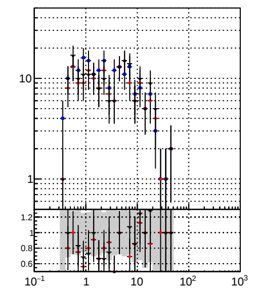
Legend: - blue diamond: Orig/DQM_orig_MS - red diamond: pixelLessOrig/DQM_mod_MS - black diamond: pixelLess/DQM_mod_MS
