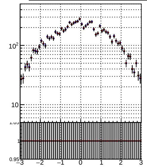
Legend: - blue diamond: Orig/DQM_orig_MS - red diamond: pixelLessOrig/DQM_mod_MS - black diamond: pixelLess/DQM_mod_MS
