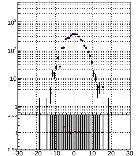
N of associated tracks (simToReco) vs z vert position
