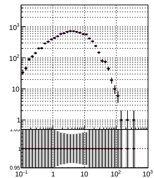
Legend: Orig/DQM_orig_MS (blue), pixelLessOrig/DQM_mod_MS (red), pixelLess/DQM_mod_MS (black)
