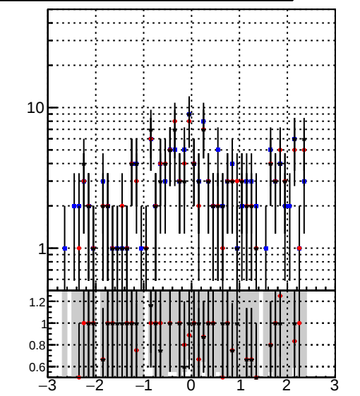
Legend: Orig/DQM_orig_MS (blue), pixelLessOrig/DQM_mod_MS (red), pixelLess/DQM_mod_MS (black)
