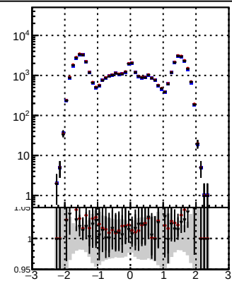
N of reco track vs \eta orig/DQM orig/MS pixelLess/DQM pixelLess/MS
