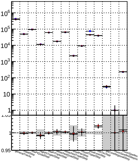
Number of tracks vs collection Legend: Orig/DQM_orig_MS pixelLessOrig/DQM_mod_MS pixelLess/DQM_mod_MS
