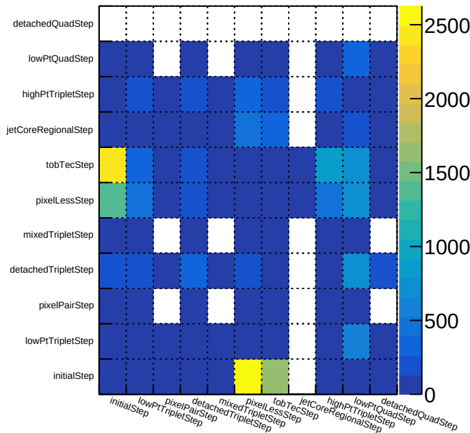
Duplicate tracks: originalAlgo vs originalAlgo
