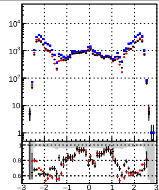
N of reco track vs \eta —•— pixelLess/DQM orig MS —•— pixelLess/DQM mod MS —•— pixelLess/DQM mod MS
