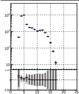
Orig/DQM orig MS pixelLessOrig/DQM mod MS N of reco track vs hit
