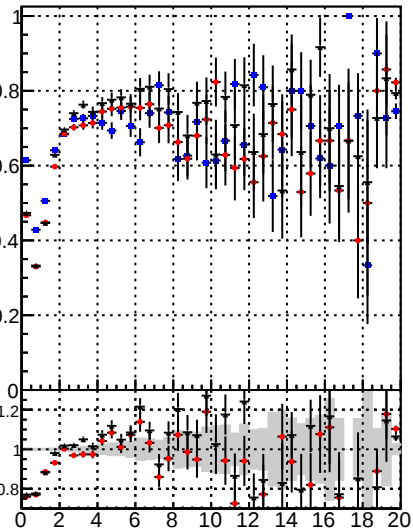
Fake rate vs. —●— Orig/DQM_orig_MS —●— pixelLessOrig/DQM_mod_MS —●— pixelLess/DQM_mod_MS
