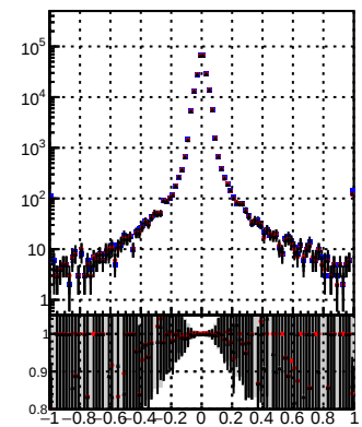
N of reco track vs dxy(PV) Legend: Orig/DQM orig MS (black dots) pixelLessOrig/DQM mod MS (red line) pixelLess/DQM mod MS (black line)
