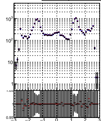
N of reco track vs \eta —●— Orig/DQM_orig_MS —■— pixelLess/DQM_mod_MS —▲— Orig/DQM_mod_MS —◆— pixelLess/DQM_orig_MS
