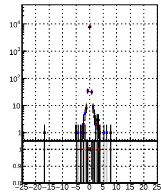
N of reco track vs dxy(PV) Orig/DQM orig MS pixelLessOrig/DQM mod MS pixelLess/DQM mod MS
