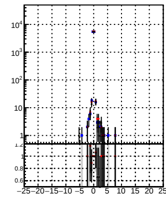
N of reco track vs dxy(PV) Orig/DQM orig MS pixelLessOrig/DQM mod MS pixelLess/DQM mod MS
