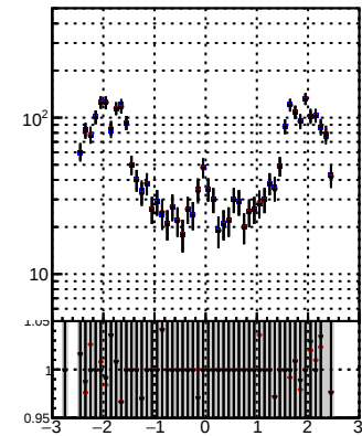
N of reco track vs \eta Orig/DQM_orig_MS pixelLess/DQM_mod_MS Orig/DQM_mod_MS pixelLess/DQM_mod_MS
