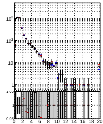
N of reco track vs. - blue circle: orig/DQM orig MS - black line: pixel Less orig/DQM mod MS - red line: pixel Less/DQM mod MS
