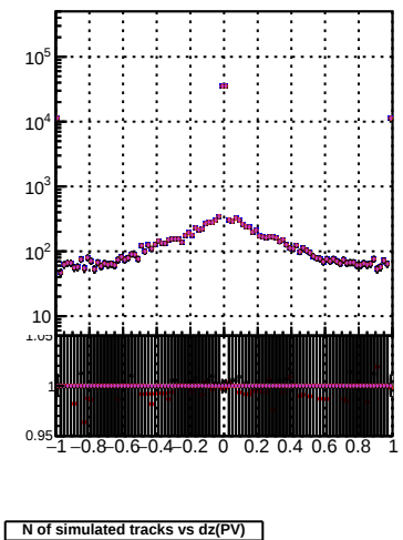
N of simulated tracks vs dz(PV)
