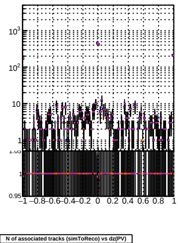
N of associated tracks (simToReco) vs dz(PV)
