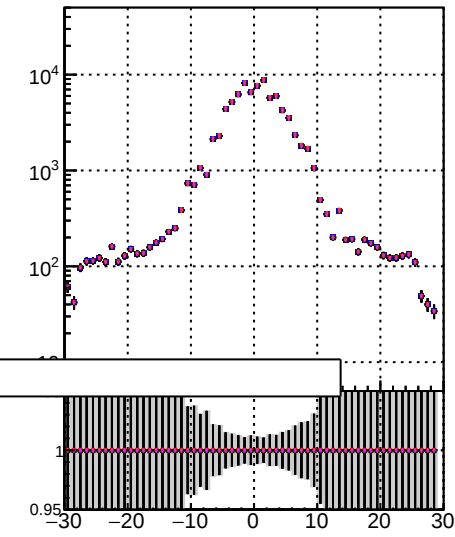
N of simulated tracks vs z vert position
