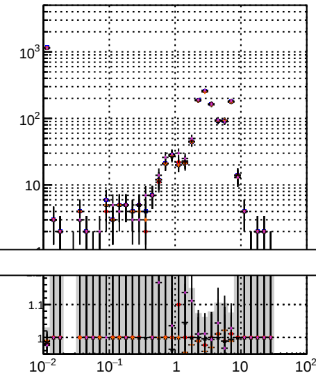
N of associated tracks (simToReco) vs transverse vert position
