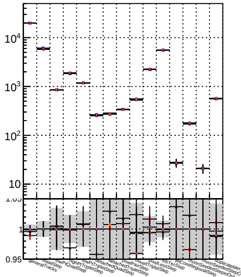
Number of tracks vs collection Legend: Original/DOM orig MS Initial/DOM orig MS highPT/Triples/DOM orig MS detachedQ/DOM orig MS detachedT/DOM orig MS
