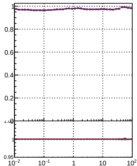
Fake rate vs v — Orig/DQM_orig_MS — higher Thr/DQM_orig_MS — detached/DQM_orig_MS
