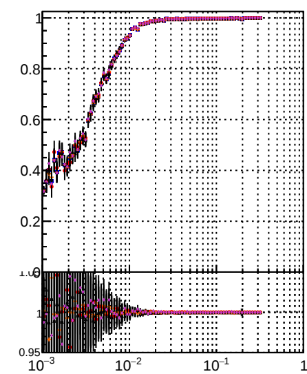
Fake rate vs Orig/DQM_orig_MS higher/DQM_orig_MS higher/DQM_orig_MS detached/DQM_orig_MS
