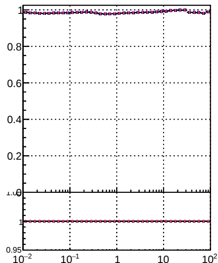
Fake rate vs v_{\text{top}} Orig/DQM_orig_MS higher/DQM_orig_MS detached/DQM_orig_MS
