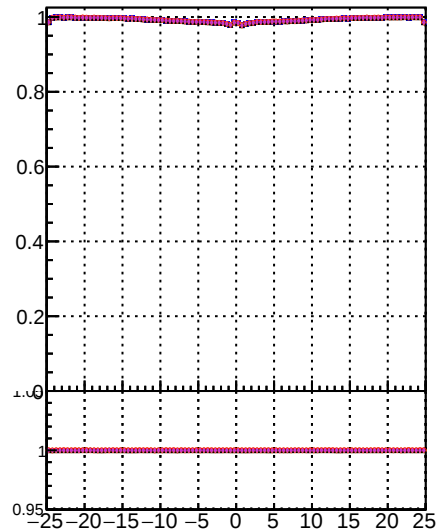
Fake rate vs d Legend: Orig/DQM_orig_MS (black circles) MultiPileupOrig_MS (red circles) detached/DQM_orig_MS (blue circles)
