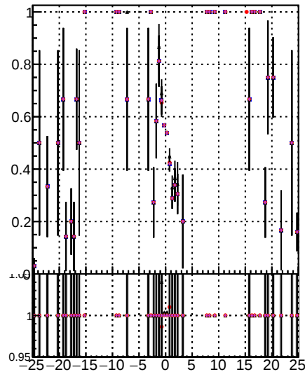
Fake rate vs d Orig/DQM_orig_MS Filtered/DQM_orig_MS detached/DQM_orig_MS
