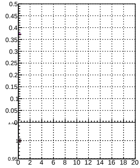
Fake rate vs. \chi^2 for different methods
