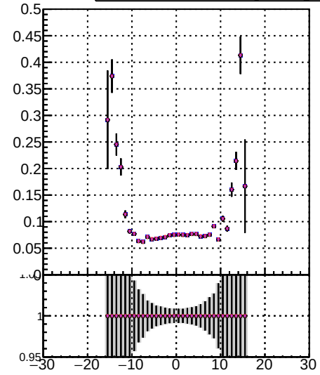
Fake rate vs \nu — Orig/DQM_orig_MS — higher/IDM/DQM_orig_MS — detached/DQM_orig_MS
