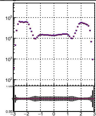
N of reco track vs \eta Orig/DQM-orig-MS recoToSim-orig-MS detached/DQM-orig-MS
