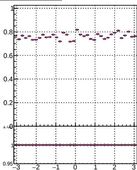
fake+duplicates vs \emptyset
