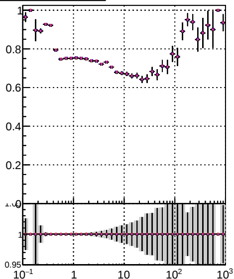
● Orig/DOM orig MS ● Initial/DOM orig MS ● highPtTriplet/DOM orig MS ● detachedO/DOM orig MS ● detachedT/DOM orig MS
