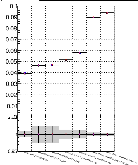
Fake rate vs. Orig/DQM_orig_MS Miniboson/DQM_orig_MS detached/DQM_orig_MS
