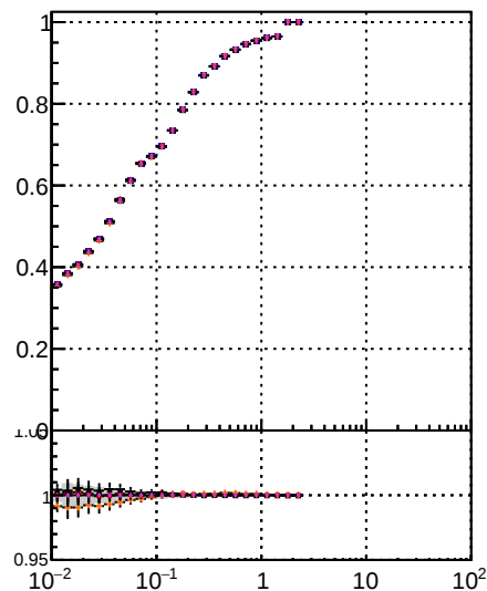
Fake rate vs v — Orig/DQM_orig_MS — Higher/DQM_orig_MS — Higher/DQM_orig_MS — detached/DQM_orig_MS
