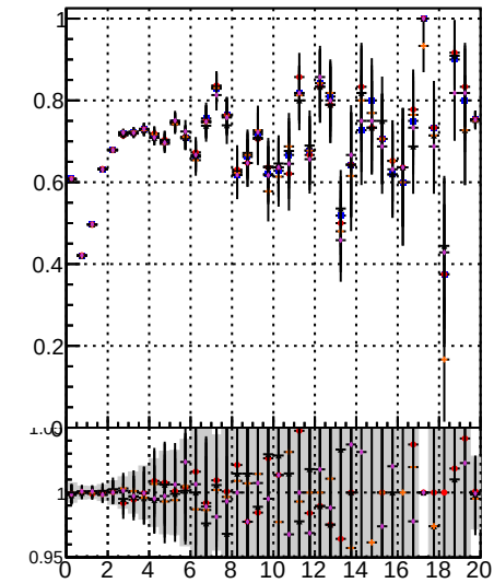
Fake rate vs. Orig/DQM_orig_MS Pileup/DQM_orig_MS Duplicates/DQM_orig_MS
