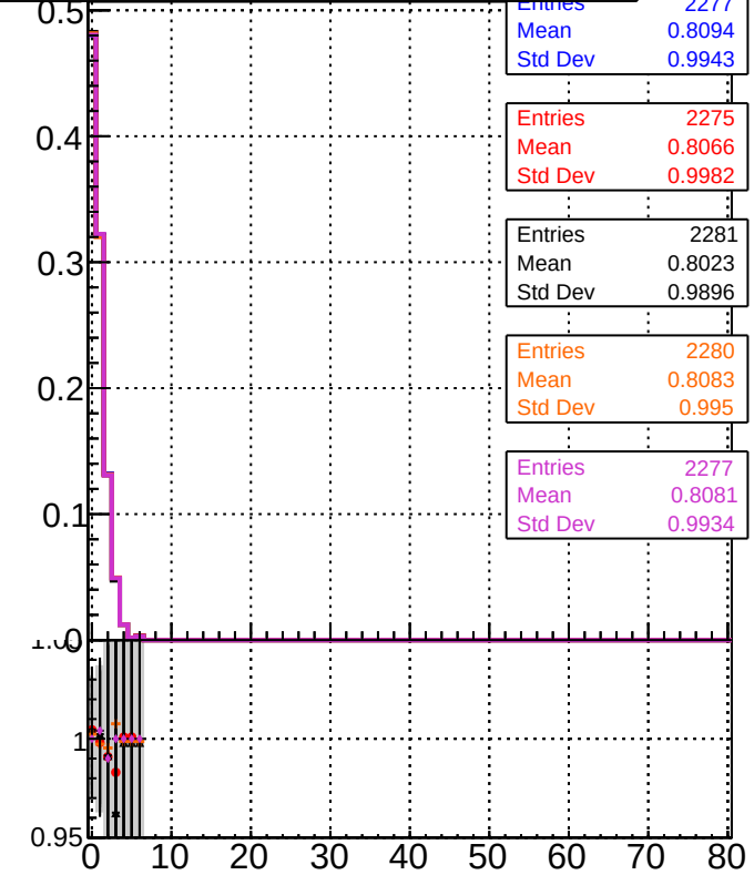
Orig/DQM_orig_MS initial/DQM_orig_MS highPtTriplet/DQM_orig_MS detachedD/DQM_orig_MS detachedT/DQM_orig_MS
