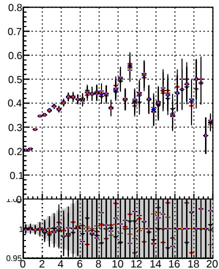
Fake rate vs. Orig/DQM_orig_MS Minibias/DQM_orig_MS Minibias/DQM_orig_MS detached/DQM_orig_MS
