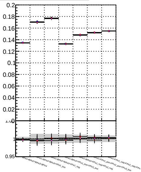
Fake rate vs. Orig/DQM_orig_MS Detached/DQM_orig_MS Detached/DQM_orig_MS Detached/DQM_orig_MS
