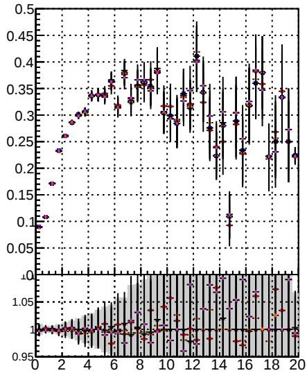
Fake rate vs. Orig/DQM_orig_MS Detached/DQM_orig_MS Detached/DQM_orig_MS Detached/DQM_orig_MS
