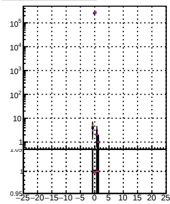
Orig/DOM orig MS N of reco track vs dxy(PV) N of associated (recoToSim) tracks vs dxy(PV) N of associated (recoToSim) loop tracks vs dxy(PV)
