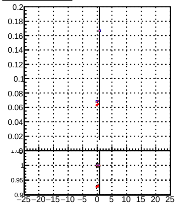
Original/DOM orig MS Initial/DOM orig MS High Pileup/DOM orig MS Detached/DOM orig MS
